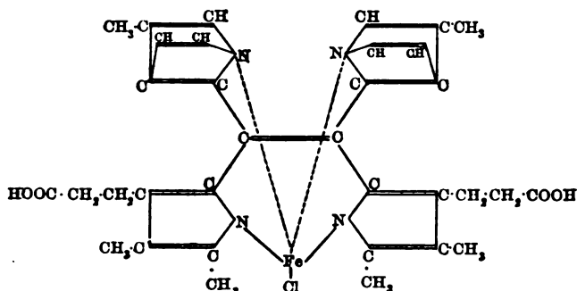
Haemin, C_{38}H_{38}O_4N_4FeCl .
